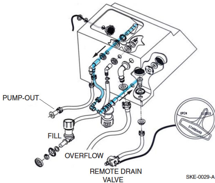
Livewell Recirculation Water Flow Figure 3-16
