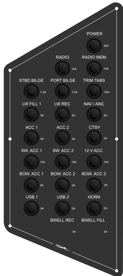
Circuit Breaker - WX1910 Figure 3-8
