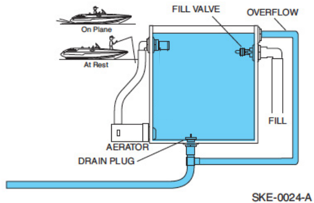
Console Livewell System Figure 3-16
