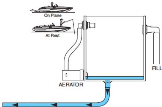
Rear Livewell System Figure 3-15
