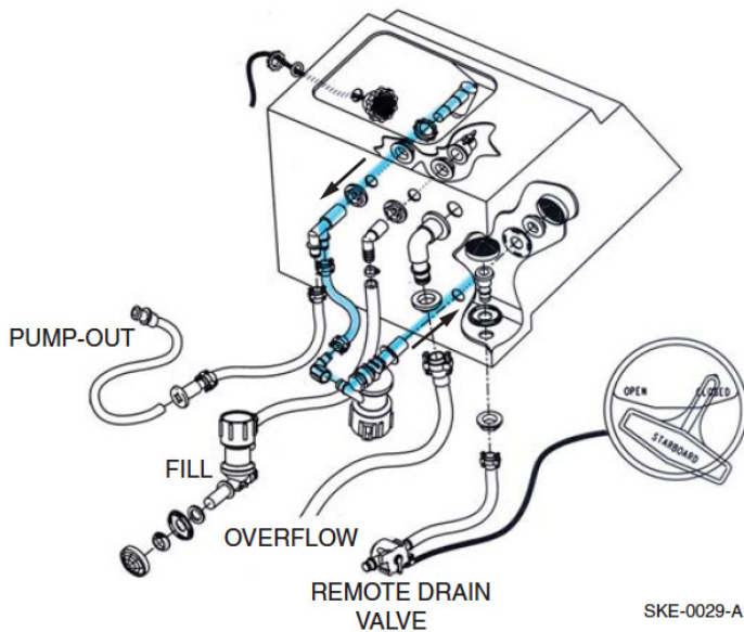
Livewell Recirculation Water Flow Figure 3-12
