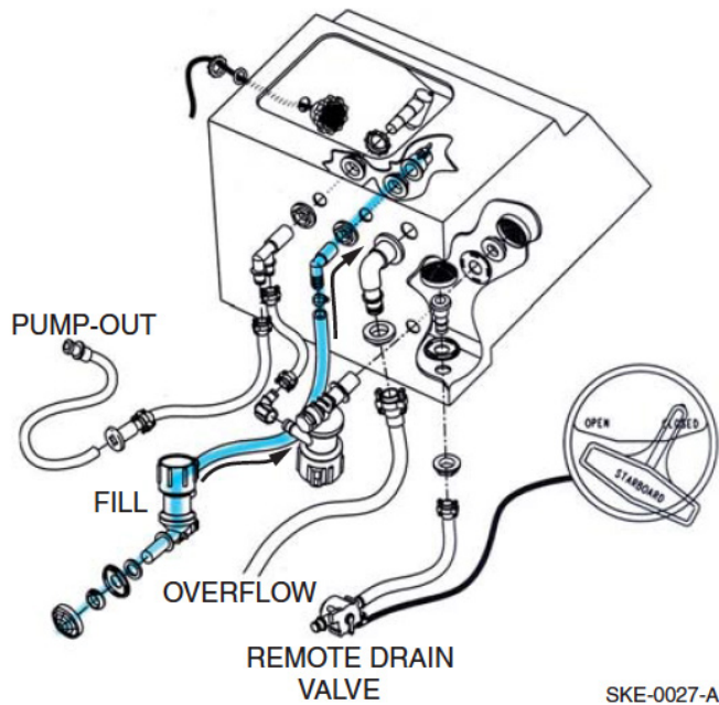
Livewell Fill Water Flow Figure 3-10
