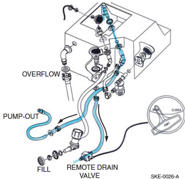
Livewell Drain Water Flow Figure 3-14
