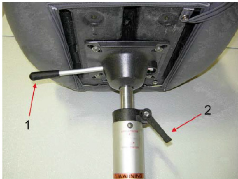
Seat Mount Figure 3-9
