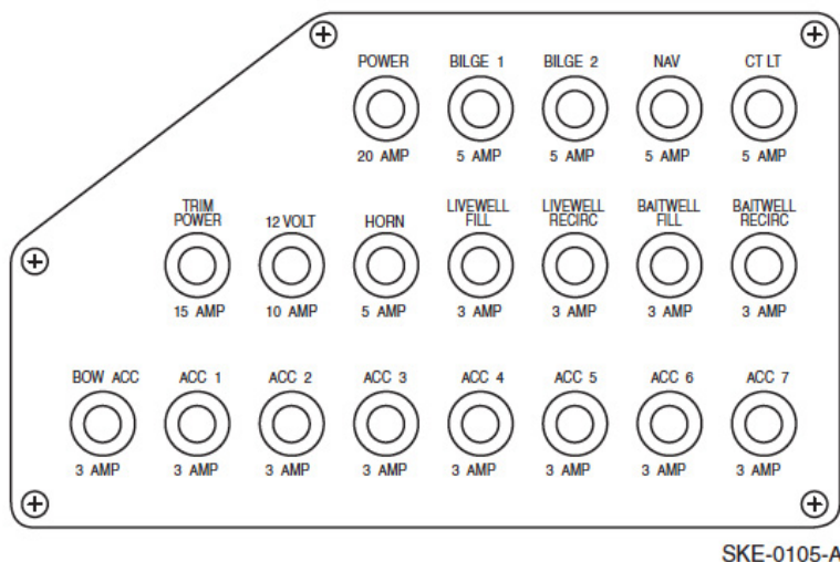
Circuit Breaker - WX1910 Figure 3-7
