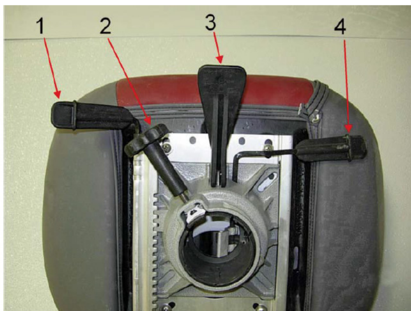
WX Series Driver's Seat Figure 3-8
