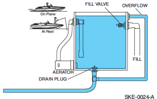
Console Livewell System Figure 3-16
