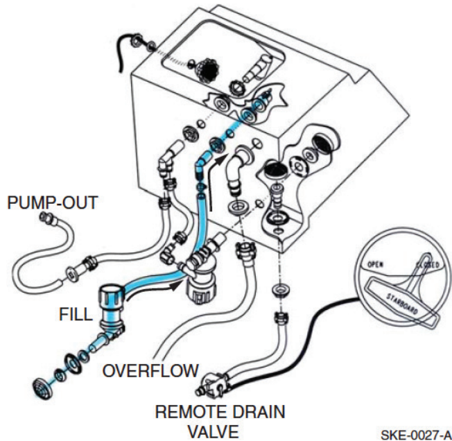
Livewell Fill Water Flow Figure 3-15
