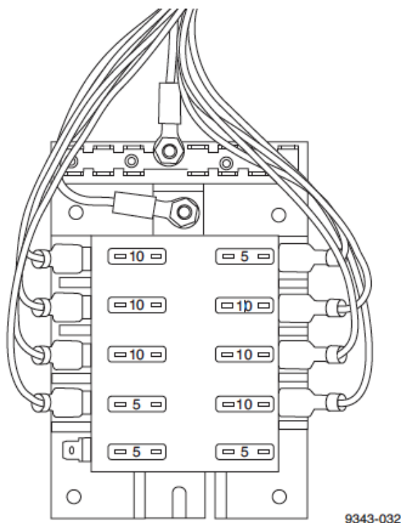
SL Fuse Panel Figure 5-3
