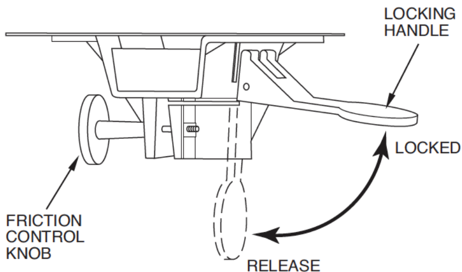
Swivel Seats Figure 5-4
