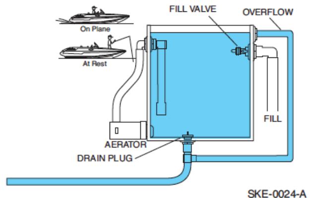
Console Livewell System Figure 3-15
